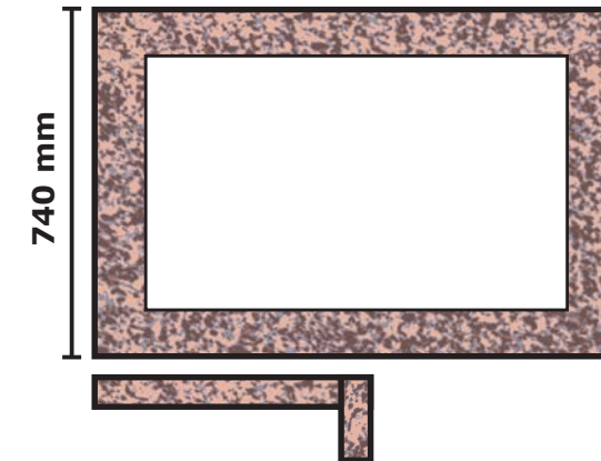
SELF SERVİS GRANİT TABLA (Hazneli Ürünler İçin) SELF SERVICE GRANITE TABLE FOR NEUTRAL PRODUCT
